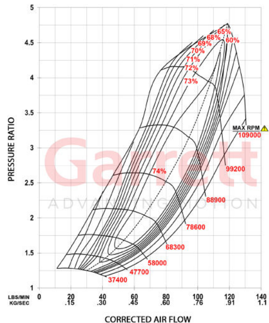
GXR45-73 Compressor Map
