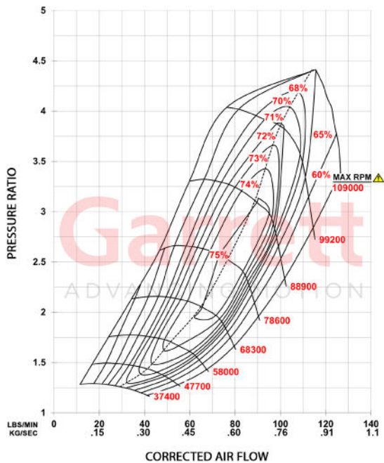
GXR42-68 Compressor Map
