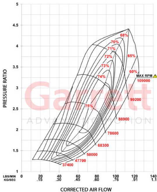
GXR45-67 Compressor Map
