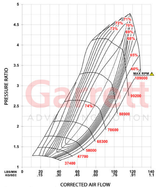
GXR42-72 Compressor Map
